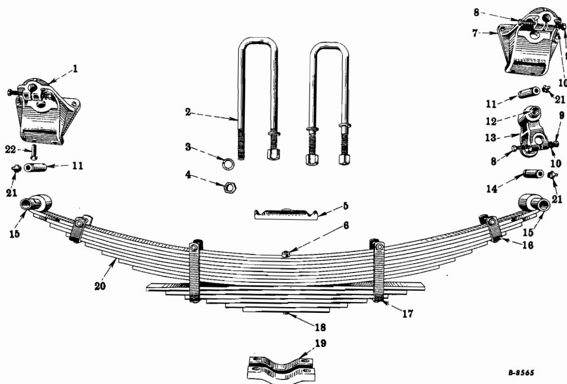
FIG. 03-12 — REAR SPRINGS, PROGRESSIVE (Code 0304) (R-153, R-163)
