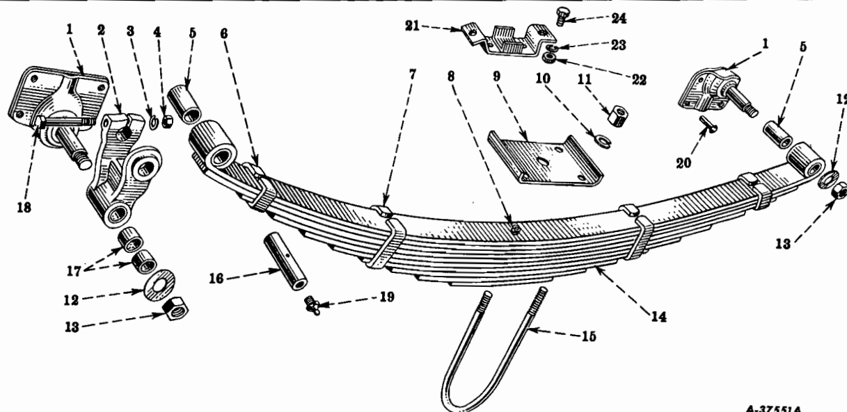
FIG. 03-8 - REAR SPRINGS
