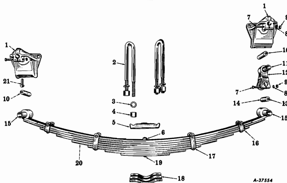
FIG. 03-14 – REAR SPRINGS (R-163)
