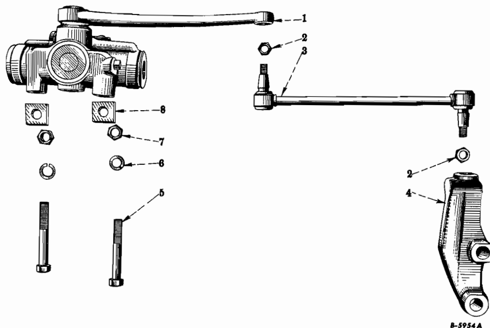
FIG. 03-20 - REAR SHOCK ABSORBERS AND MOUNTING (Code 0303) (R-140-4x4, R-150, R-160-4x4, R-160, RC-160 Series)
