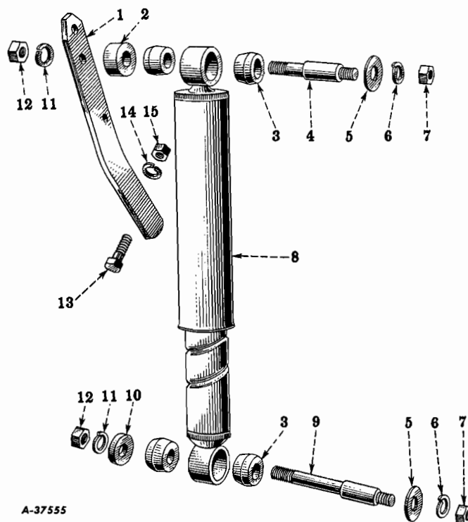
FIG. 03-15 - FRONT SHOCK ABSORBERS (R-130 Series)
