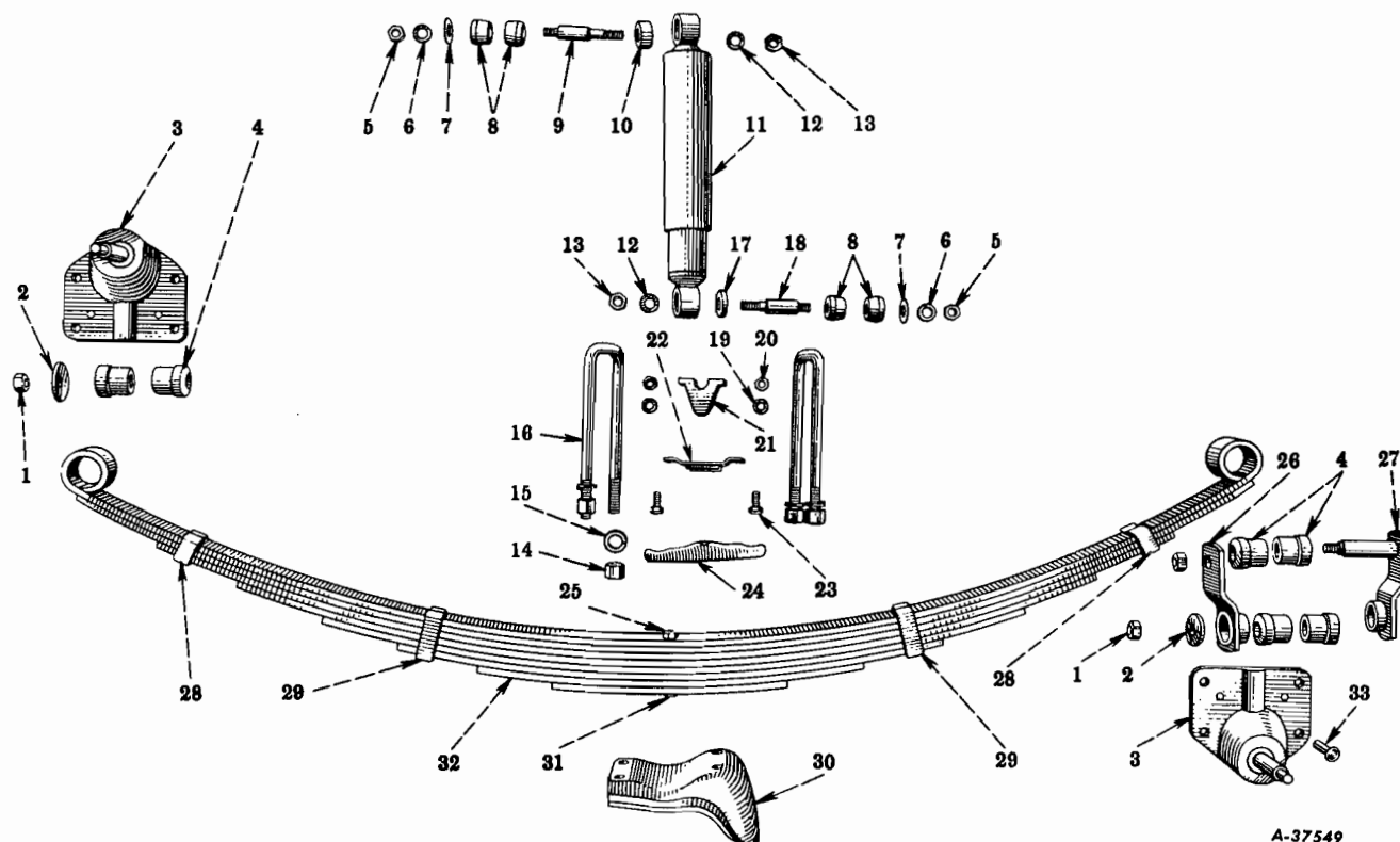
FIG. 03-6 - REAR SPRINGS AND SHOCK ABSORBERS (Without Auxiliary Springs) (R-110 Series - With Standard Springs; Chassis No. 501 to 31543 And Chassis No. 47867 Up) (R-110 Series - With Heavy-Duty Springs, Code 0307) (R-120 Series)
