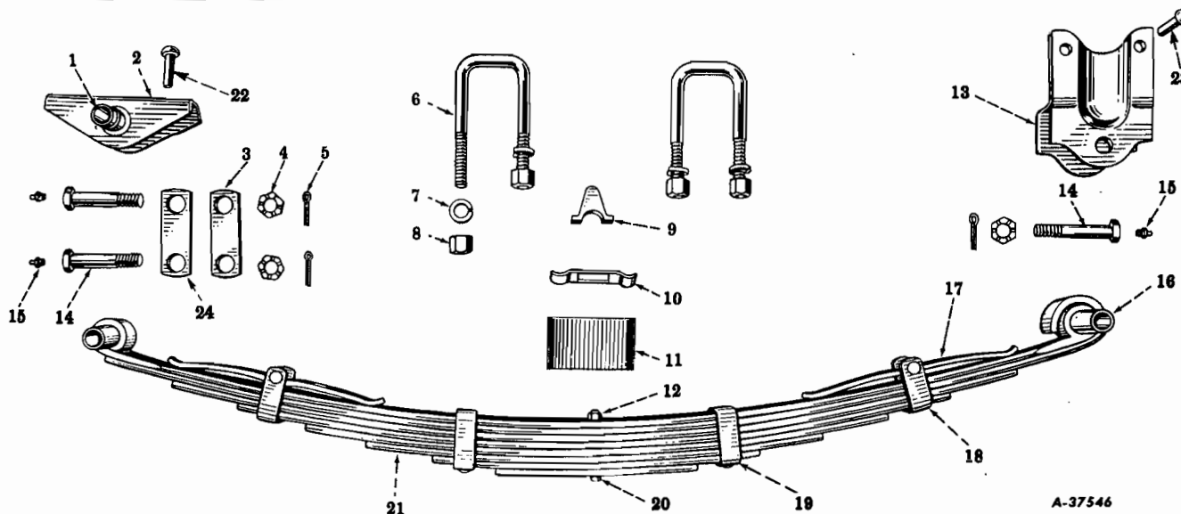
FIG. 03-3 - FRONT SPRINGS (R-150, R-160, RC-160 Series)
