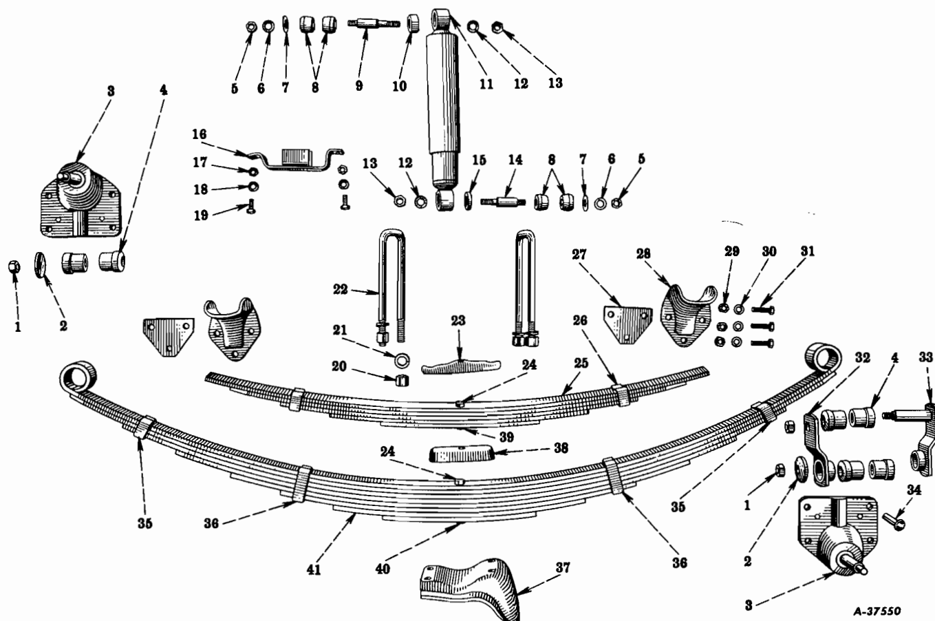
FIG. 03-7 — REAR SPRINGS AND SHOCK ABSORBERS (With Auxiliary Springs, Code 0301) (R-110 Series - With Standard Springs; Chassis No. 501 To 31543 And Chassis No. 47867 Up) (R-110 Series - With Heavy-Duty Springs, Code 0307) (R-120 Series)
