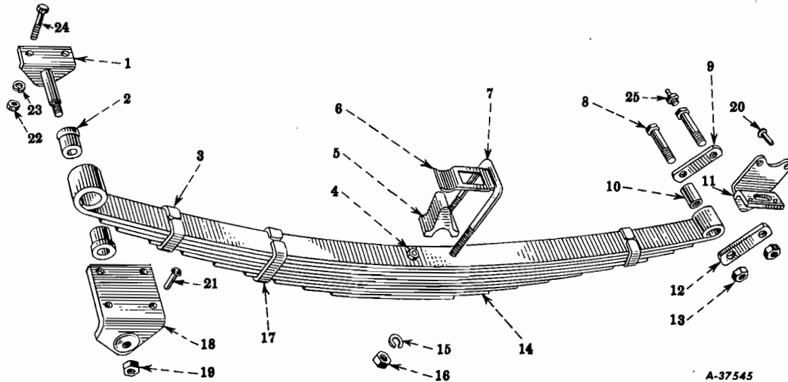
FIG. 03-2 - FRONT SPRINGS (R-130 Series)
