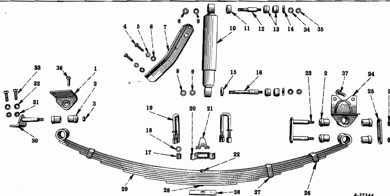
FIG. 03-1 - FRONT SPRINGS AND SHOCK ABSORBERS (R-100, R-110, R-120 Series)
