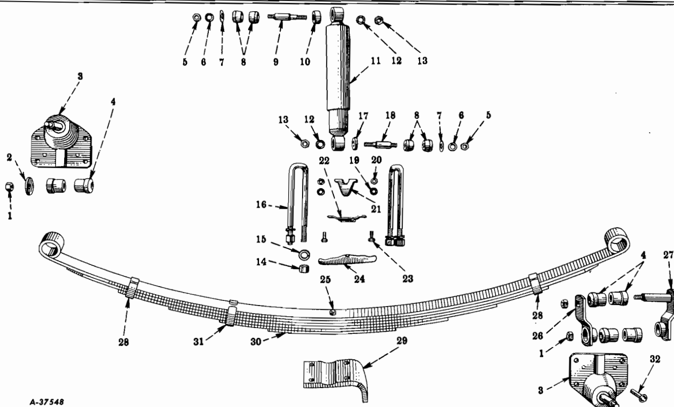
FIG. 03-5 - REAR SPRINGS (R-100 Series) (R-110 Series - With Standard Springs, Chassis No. 31544 to 47866)
