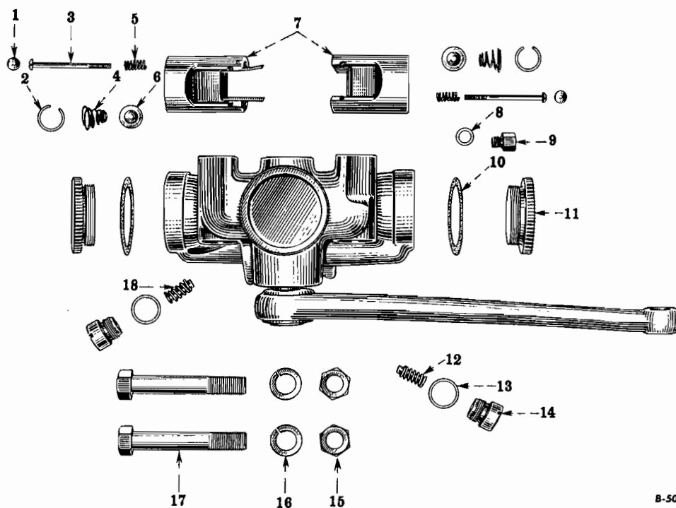
FIG. 03-19 — REAR SHOCK ABSORBERS (Code 0303) (R-140-4x4, R-150, R-160, R-160-4x4, RC-160)
