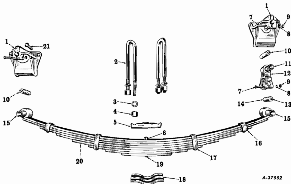
FIG. 03-10 - REAR SPRINGS (Standard And Heavy-Duty, Code 0307) (R-150 Series)
