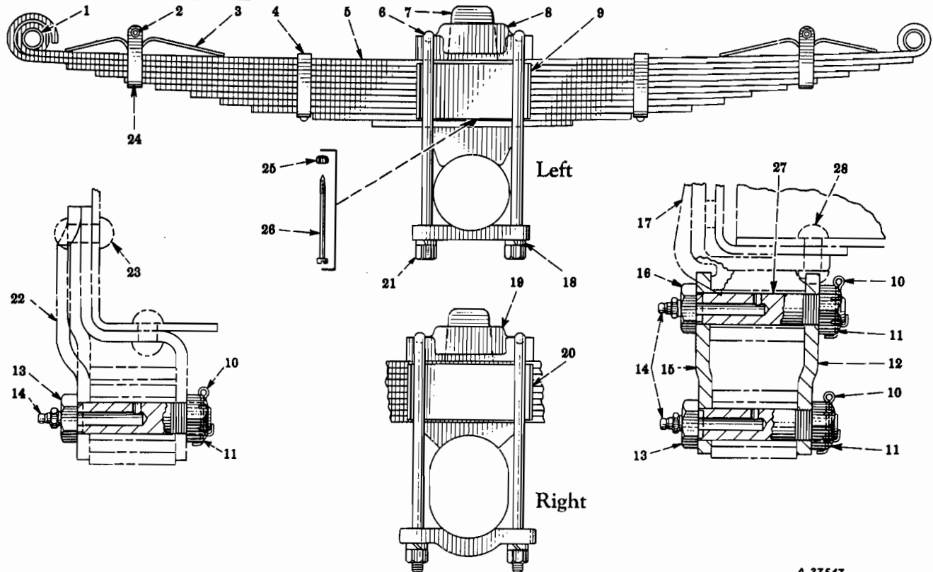
FIG. 03-4 - FRONT SPRINGS (R-140-4x4, R-160-4x4 Series)
