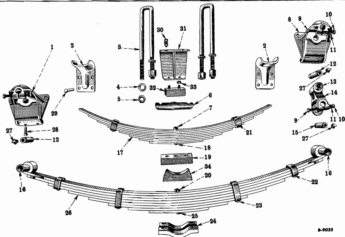
FIG. 03-13 - REAR AND AUXILIARY SPRINGS (R-140-4x4, R-160, R-164, R-165, R-160-4x4, RC-160 Series)
